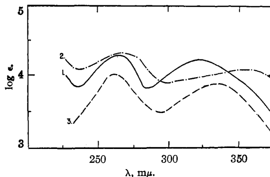
Fig. 10.—Ultraviolet spectra: 1, desoxydesdimethylaminoterramycin in acid-ethanol; 2, Terramycin in acid-ethanol; 3, 8-hydroxy-1-tetralone in acid-ethanol + 3,6-dihydroxy-4-keto-2,5-cholestadiene (xxvi) in chloroform (latter calculated from Windaus and Kuhr, ref. 37.)
