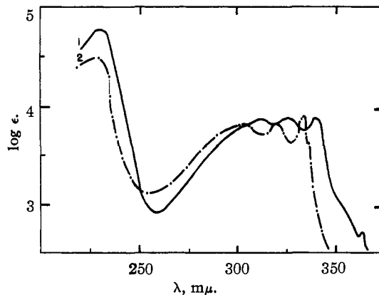
Fig. 3.—Ultraviolet spectra: 1, terrannaphthol in ethanol; 2, 1,8-naphthalenediol in ethanol.
