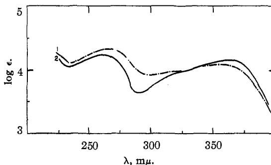
Fig. 11.—Ultraviolet spectra in acid-ethanol: 1, Terramycin; 2, desdimethylaminoterramycin.
