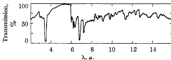
Fig. 2.—Infrared spectrum of Terramycin mullied in mineral oil.
