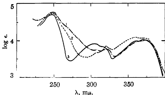
Fig. 7.—Ultraviolet spectra in acid-ethanol: 1, \beta -apoterramycin; 2, terrinolide; 3, decarboxamidoterrinolide.
