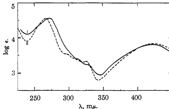
Fig. 5.—Ultraviolet spectra in acid-ethanol: 1, anhydroterramycin; 2, 8,9,10-trihydroxy-1-keto-1,2,3,4-tetrahydroanthracene.
