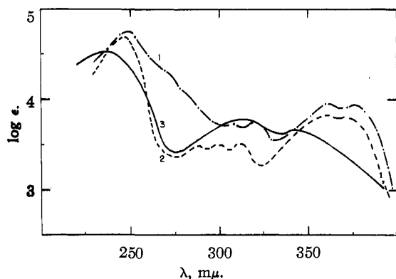
Fig. 6.—Ultraviolet spectra in acid-ethanol: 1, \beta -apoterramycin; 2, 1,8-dihydroxy-2-naphthoic acid (XXXI); 3, terranaphthoic acid (XXXII).
