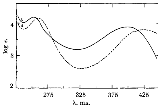
Fig. 8.—Ultraviolet spectra in concentrated sulfuric acid: 1, 3-methoxy-6-methylpyromellitic anhydride; 2, dimethoxypyromellitic anhydride, replotted from reference 25.
