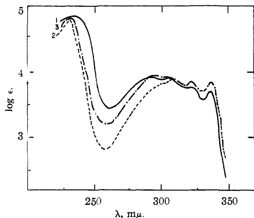
Fig. 9.—Ultraviolet spectra in ethanol: 1, the glycol XLI; 2, terranaphthol; 3, terranaphthol + 1,2,4-trimethoxybenzene.
