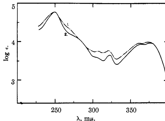
Fig. 12.—Ultraviolet spectra in acid-ethanol: 1, \beta -apoterracycin; 2, \alpha -apoterracycin.
