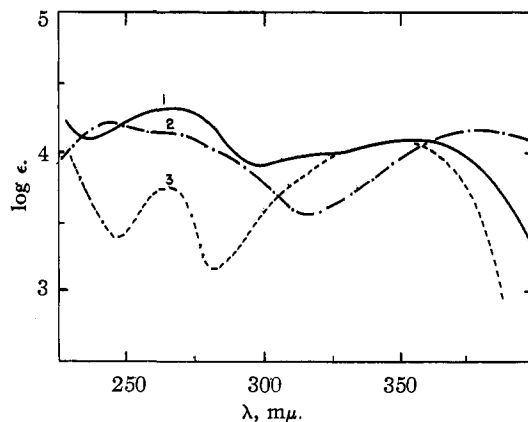
Fig. 1.—Ultraviolet spectra: 1, Terramycin in acid-ethanol; 2, Terramycin in alkaline ethanol; 3, 2-acetyl-8-hydroxytetralone (XXIV) in acid-ethanol.
